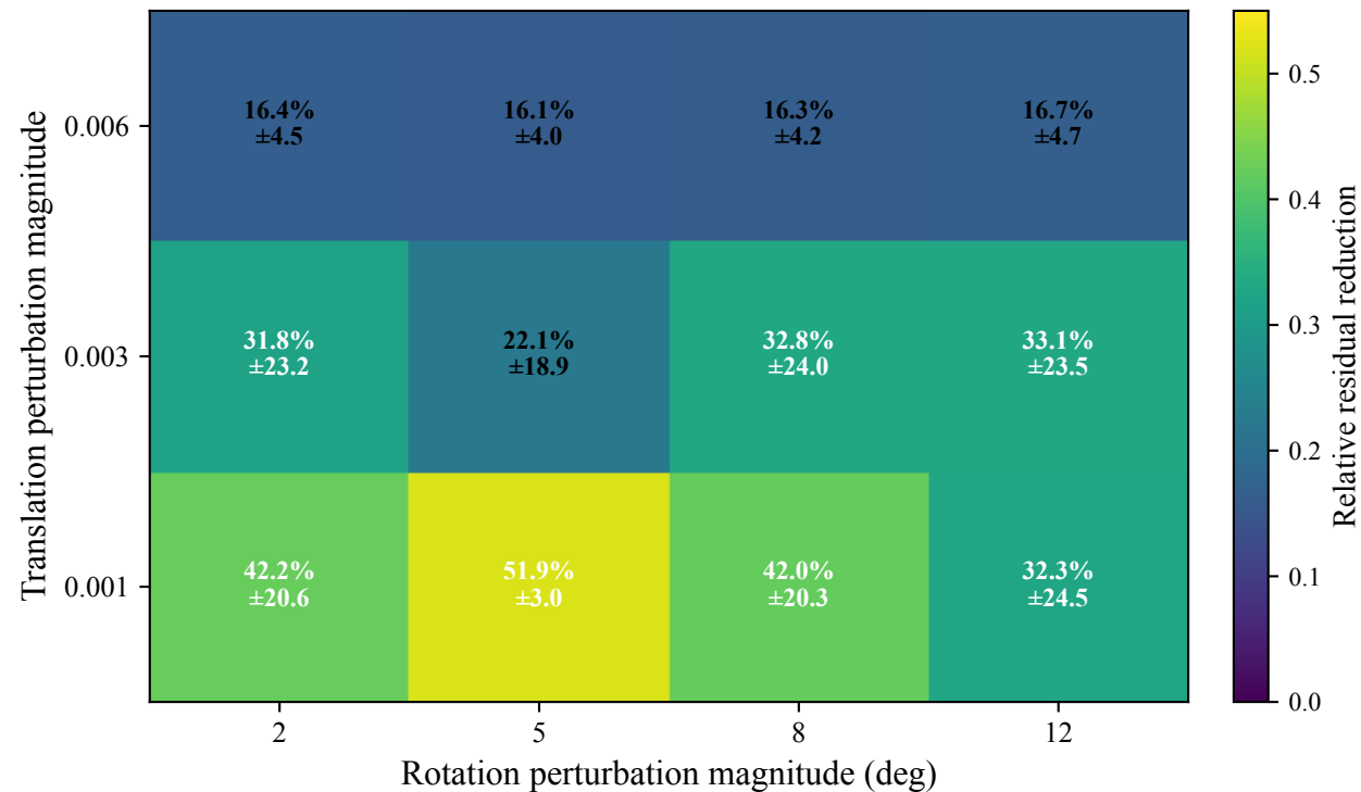
Mean Residual Reduction under Different Initializations
